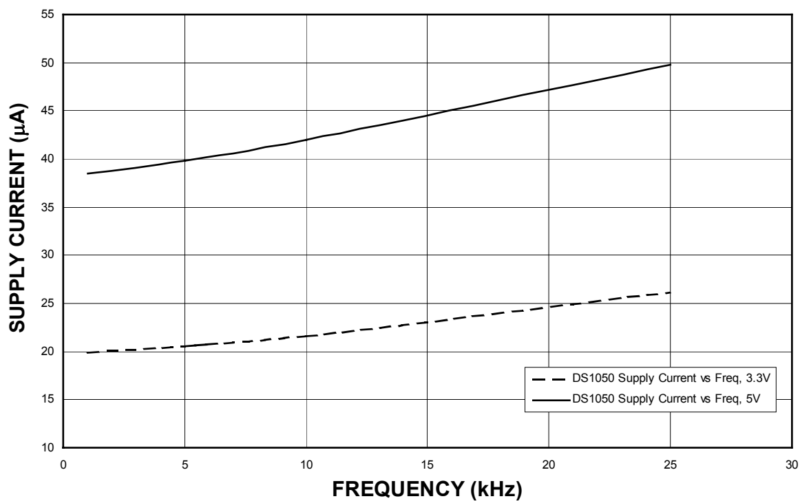
DS1050 SUPPLY CURRENT vs. FREQUENCY
