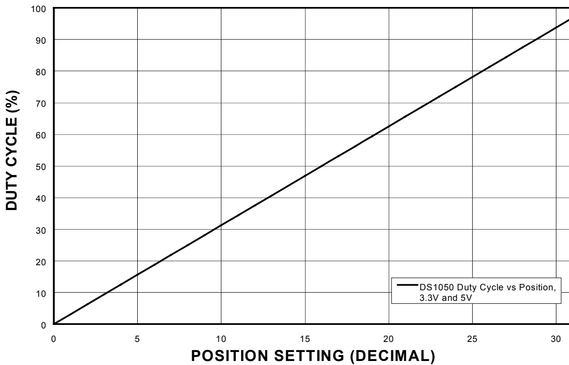
DS1050 DUTY CYCLE vs. POSITION
