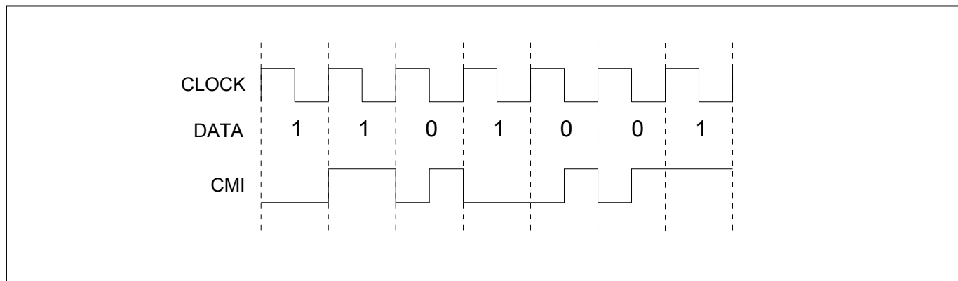
Figure 23-2. CMI Coding
