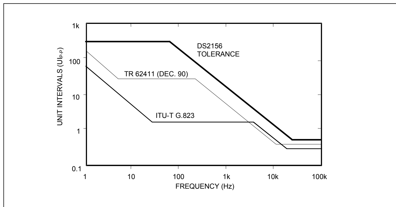
Figure 23-7. Jitter Tolerance
