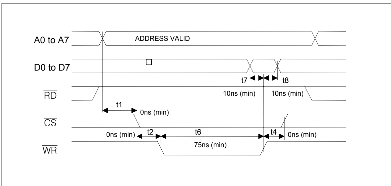
Figure 36-5. Intel Bus Write Timing (BTS = 0/MUX = 0)
