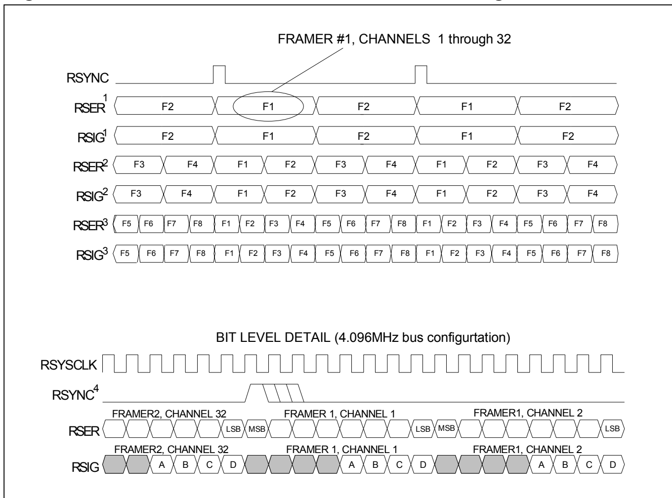
Figure 34-16. Receive IBO Frame Interleave Mode Timing
