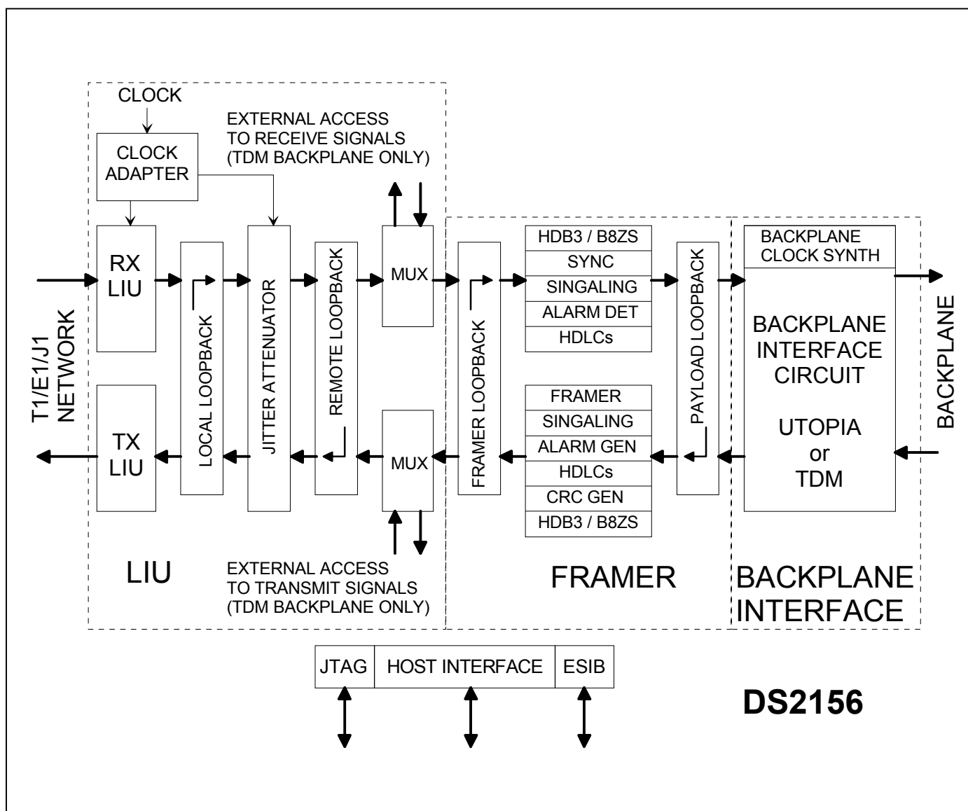
Figure 2-1. Block Diagram
