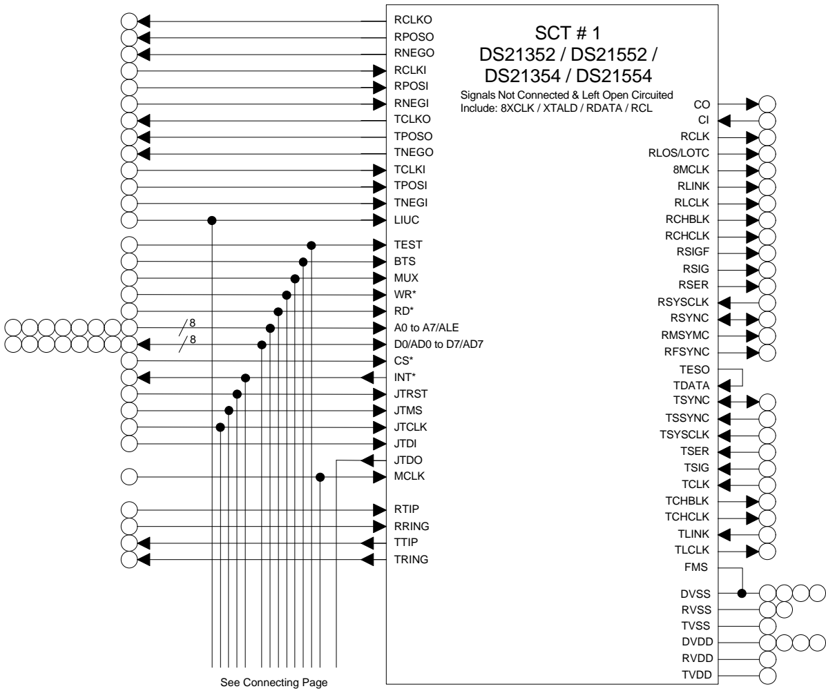
DS21Q352 / DS21Q552 / DS21Q354 / DS21Q554 Schematic Figure 1
