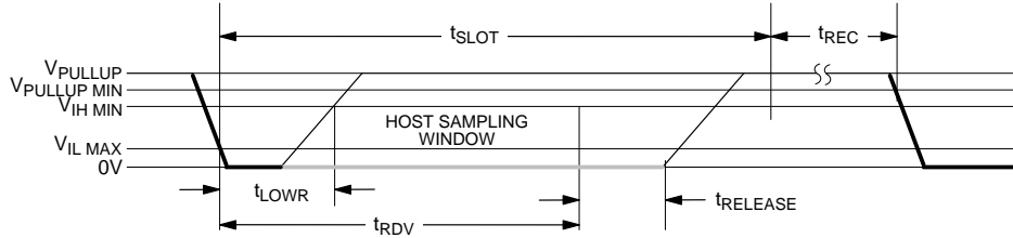
Read-Data Time Slot Figure 3
