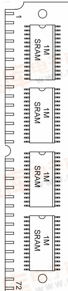
72-Pin SIP STIK
