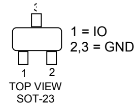
SOT-23 (3-pin) PACKAGE
