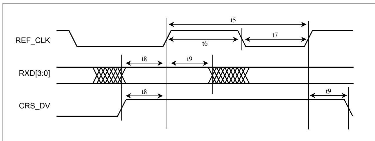
Figure 11-4 Receive RMII Interface Timing
