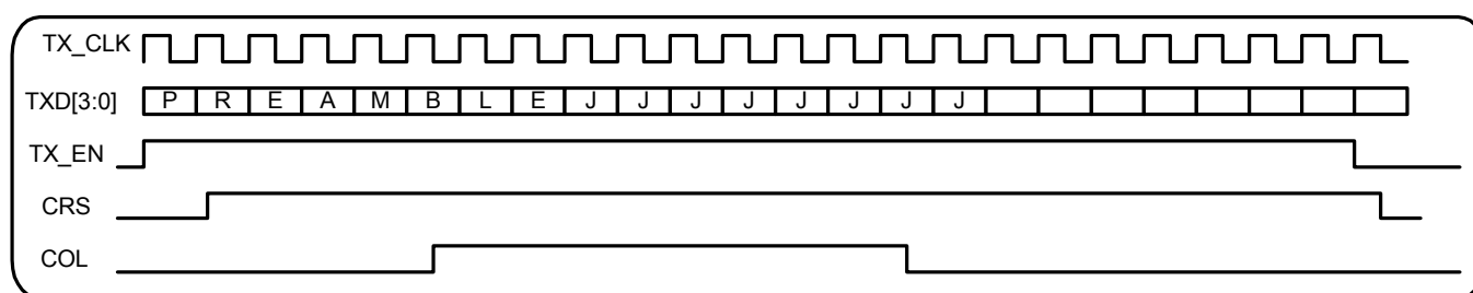
Figure 10-6 MII Transmit Half Duplex with a Collision Functional Timing
