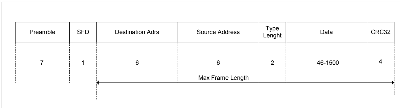
Figure 8-6. IEEE 802.3 Ethernet Frame
