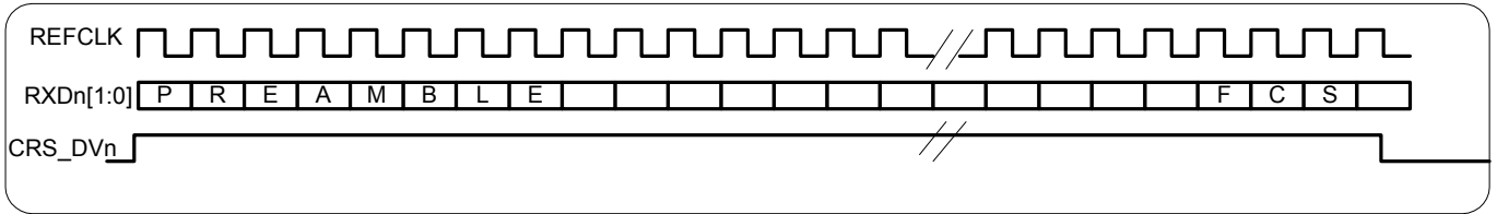
Figure 10-9. RMI Receive Interface Functional Timing
