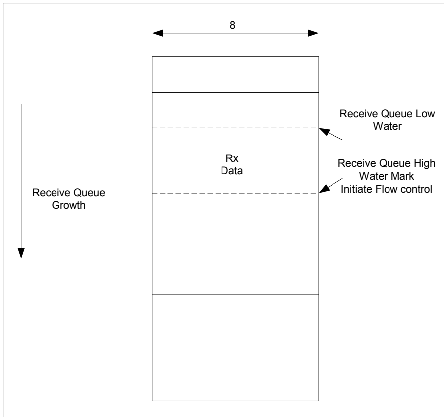
Figure 8-5. Flow Control Using Pause Control Frame
