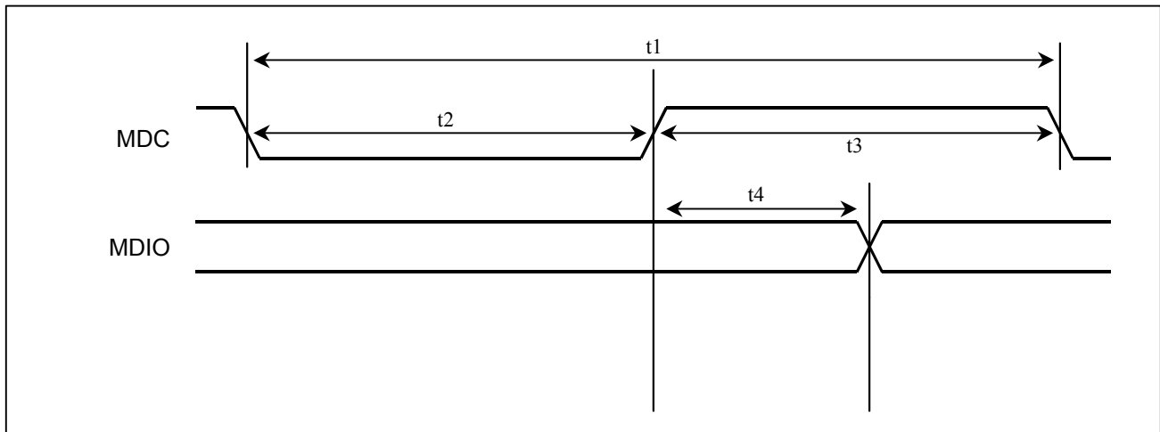
Figure 11-5. MDIO Timing
