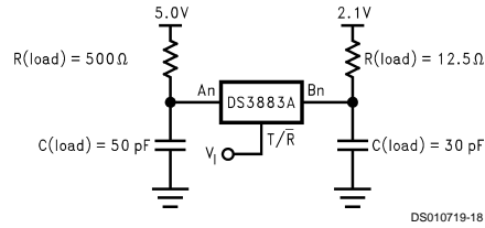
FIGURE 8. T/\bar{R} to An, T/\bar{R} to Bn
