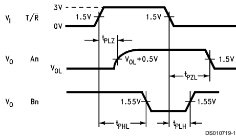
FIGURE 9. T/\bar{R} to Bn ( t_{PHL} and t_{PLH} only), T/\bar{R} to An ( t_{PZL} and t_{PLZ} only)
