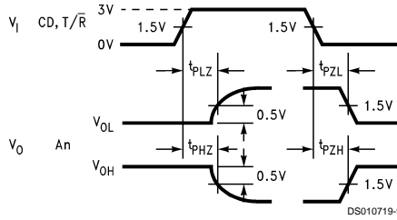
FIGURE 7. Receiver: CD to An, T/\bar{R} to An ( t_{PHZ} and t_{PZH} only)
