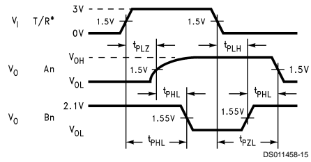
FIGURE 11. T/\bar{R} to Bn ( t_{PHL} and t_{PLH} only), T/\bar{R} to An ( t_{PZH} and t_{PZL} only)
