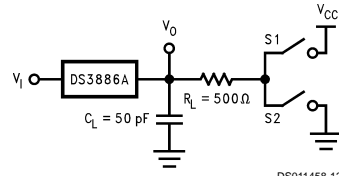
FIGURE 7. Receiver Enable/Disable Set-up
