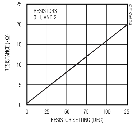
RESISTANCE vs. RESISTOR SETTING
