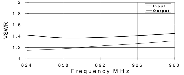
VSWR vs. Frequency
