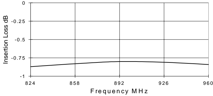
Insertion Loss vs. Frequency
