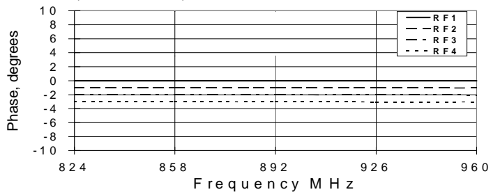
Phase Balance vs. Frequency
