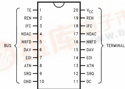
Dual-In-Line Package
