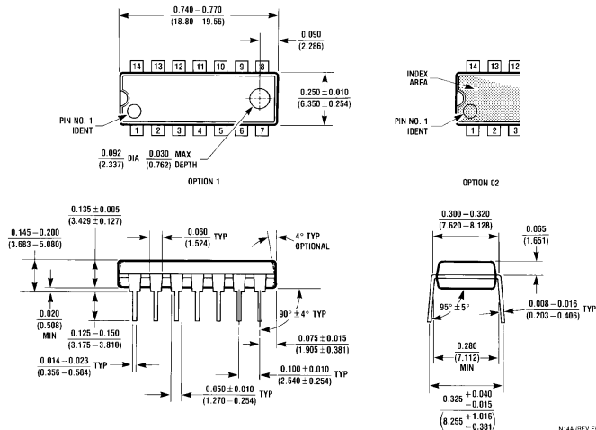
Molded Dual-In-Line Package (N) Order Number DS8640N NS Package Number N14A
