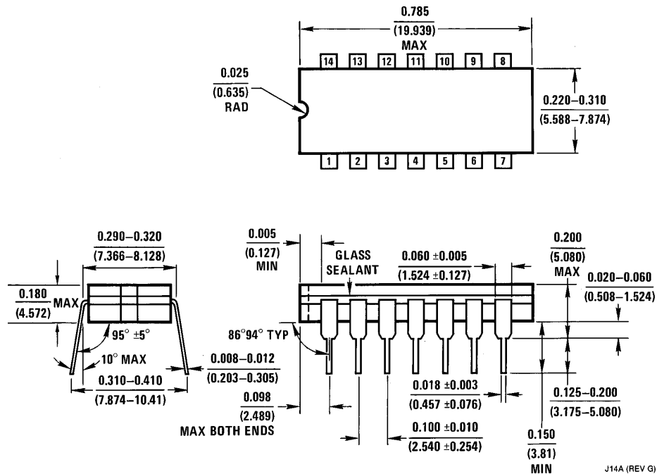
Ceramic Dual-In-Line Package (J) Order Number DS7820J NS Package Number J14A
