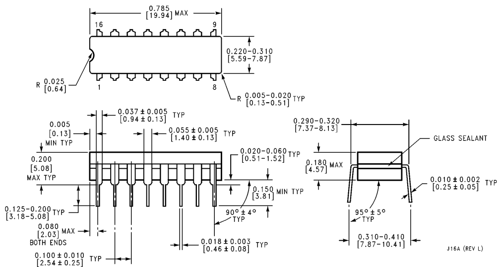
Ceramic Dual-In-Line Package (J) Order Number DS7837J NS Package Number J16A
