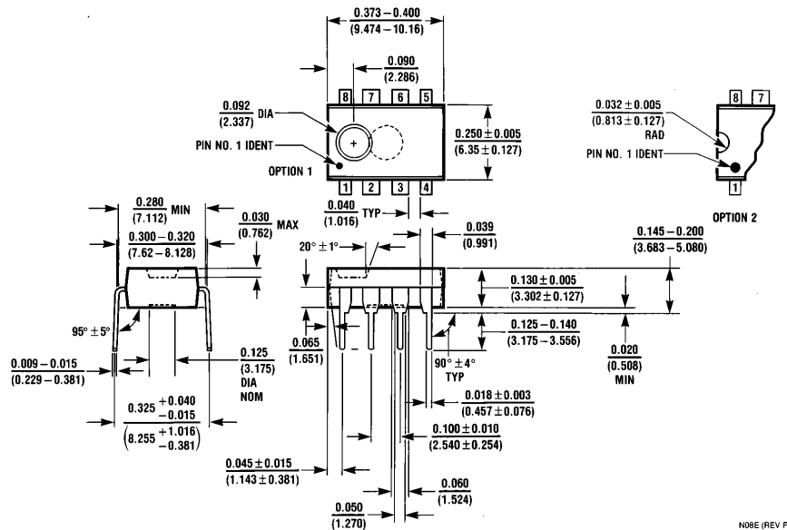
Molded Dual-In-Line Package (N) Order Number DS8614N, DS8615N, DS8616N or DS8617N (-4, -3, -2) NS Package Number N08E
