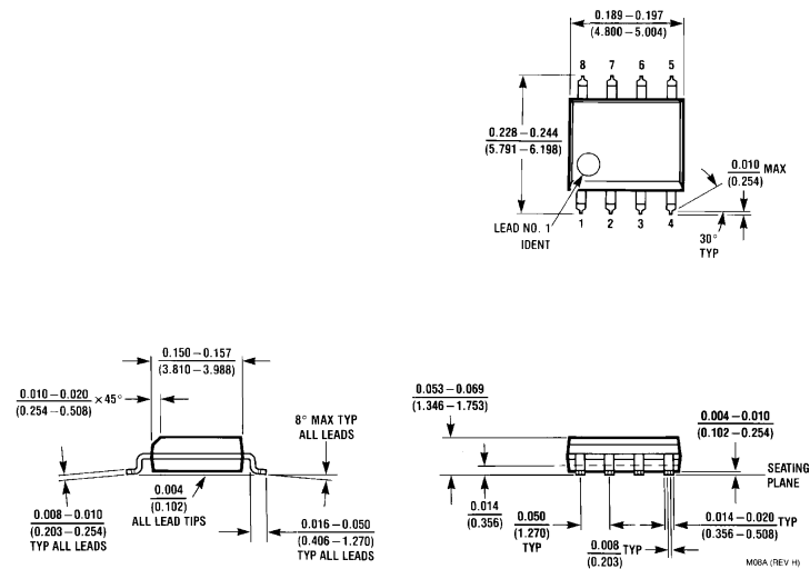
Molded Dual-In-Line Package (M) Order Number DS8614M-4, DS8615M-4, DS8616M-4 or DS8617M-4 NS Package Number M08A
