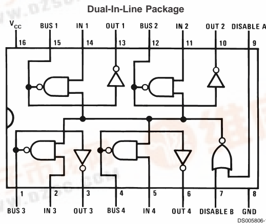
Top View Order Number DS8641N See NS Package Number N16A
