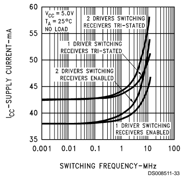
I_{CC} vs Driver Switching Frequency
