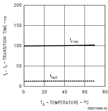
Driver Transition Time vs Temperature
