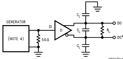
FIGURE 2. Driver Propagation Delay Test Circuit
