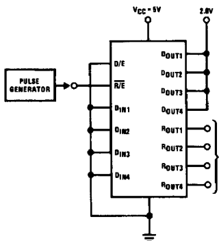
FIGURE 4. Propagation Delay (Receive/Enable to Receive Output)
