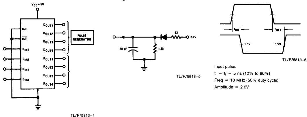
FIGURE 1. Propagation Delay ( D_{OUT} to R_{OUT} )
