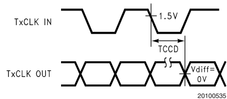
FIGURE 8. DS90C365A (Transmitter) Clock In to Clock Out Delay with R_FB pin = GND
