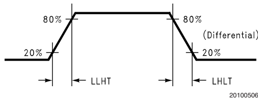
FIGURE 4. DS90C365A (Transmitter) LVDS Transition Times
