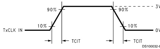
FIGURE 4. DS90CF363 (Transmitter) Input Clock Transition Time
