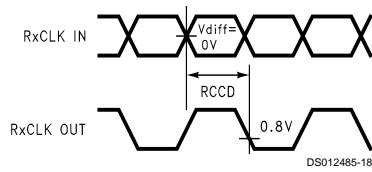
FIGURE 10. DS90CF562 (Receiver) Clock In to Clock Out Delay
