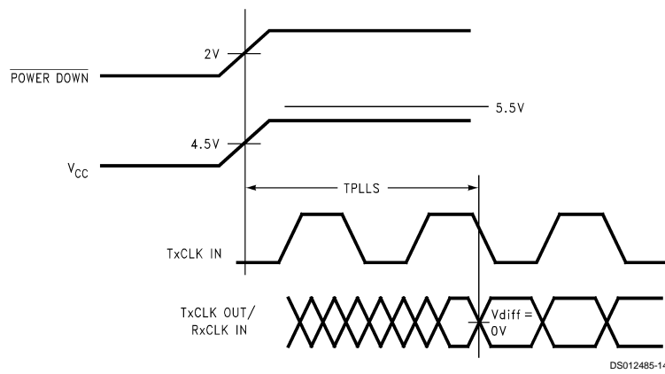
FIGURE 11. DS90CF561 (Transmitter) Phase Lock Loop Set Time
