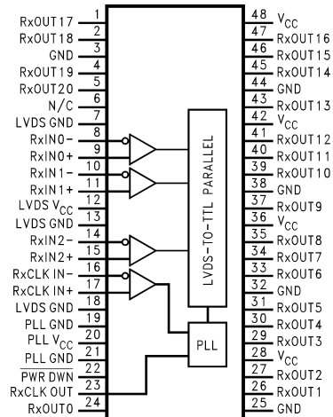
DS90CR218
