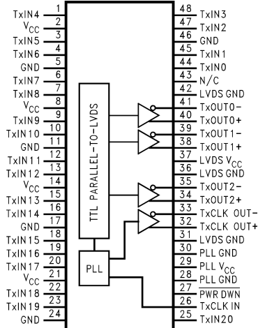
DS90CR217
