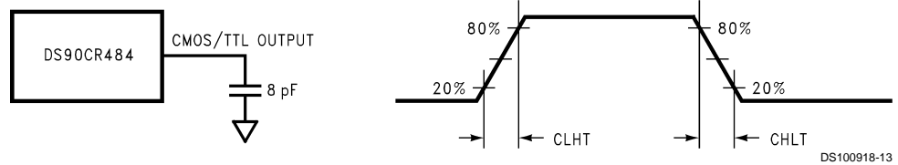
FIGURE 3. DS90CR484 (Receiver) CMOS/TTL Output Load and Transition Times
