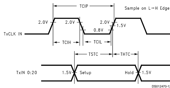
FIGURE 7. DS90CR561 Setup/Hold and High/Low Times
