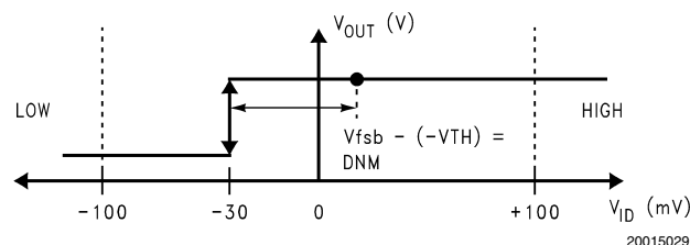
FIGURE 5. VTC of the DS90LV012A and DS90LT012A LVDS Receivers
