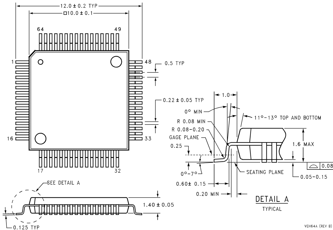
64-Lead Molded TQFP Package Order Number DS92LV090ATVEH NS Package Number VEH064DB
