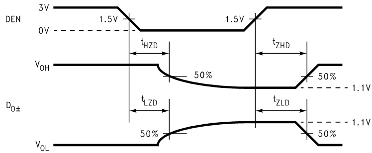
FIGURE 8. Serializer TRI-STATE Test Circuit and Timing
