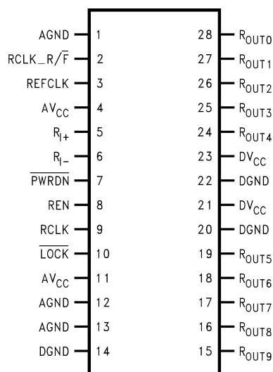
DS92LV1224TMSA - Deserializer
