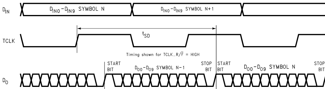
FIGURE 11. Serializer Delay
