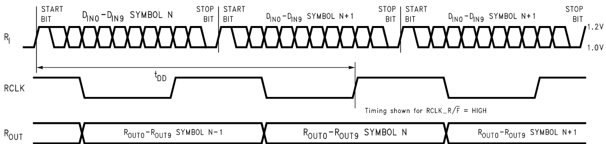
FIGURE 12. Deserializer Delay
