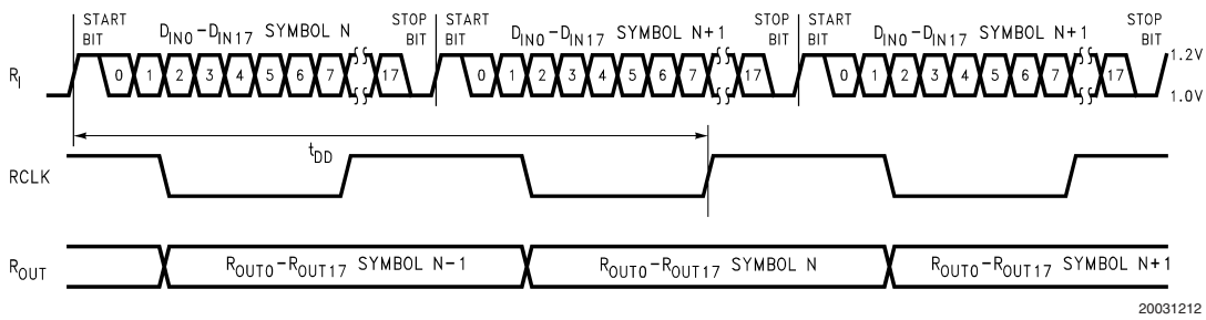
FIGURE 11. Deserializer Delay
