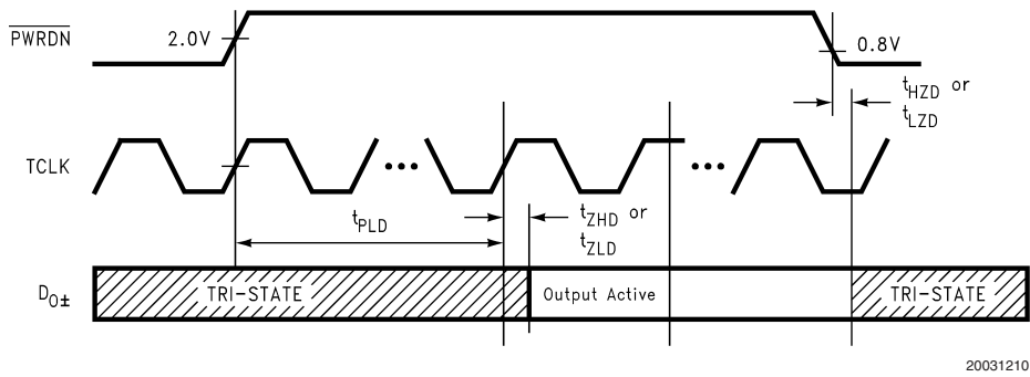
FIGURE 8. Serializer PLL Lock Time, and PWRDN TRI-STATE Delays
