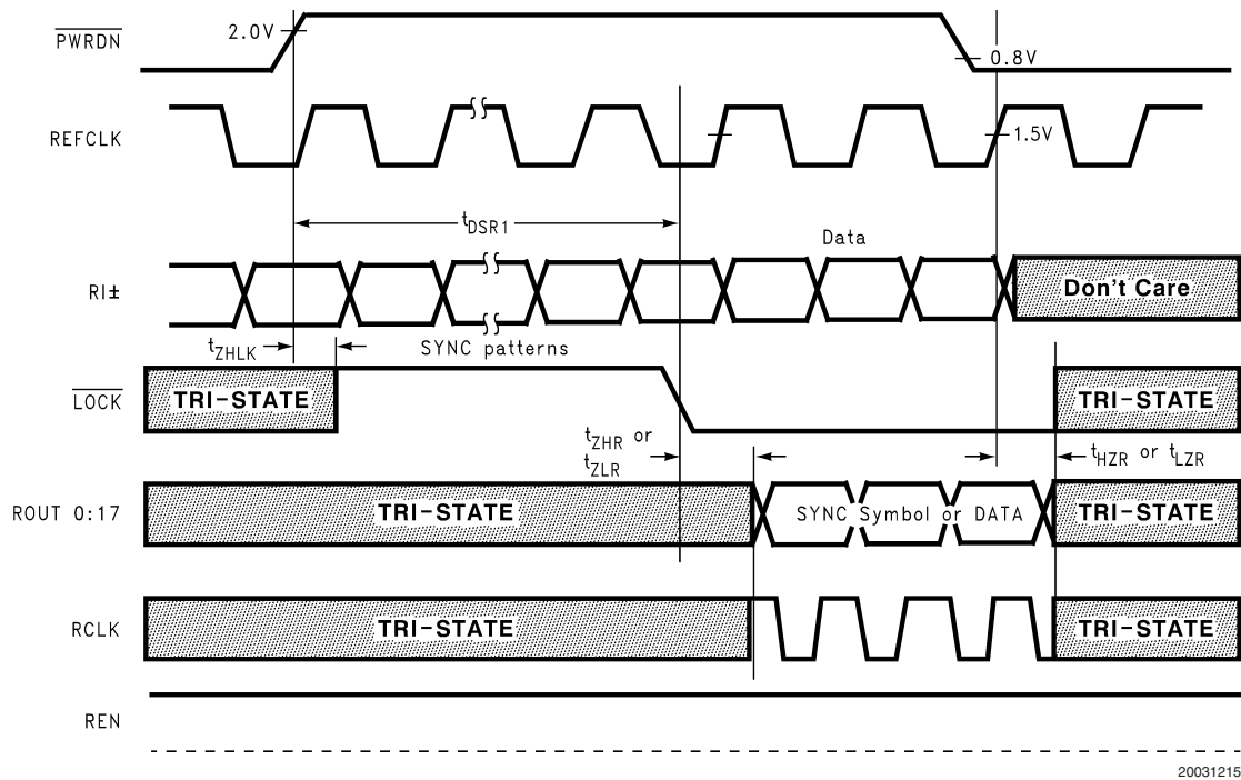
FIGURE 14. Deserializer PLL Lock Times and PWRDN TRI-STATE Delays
