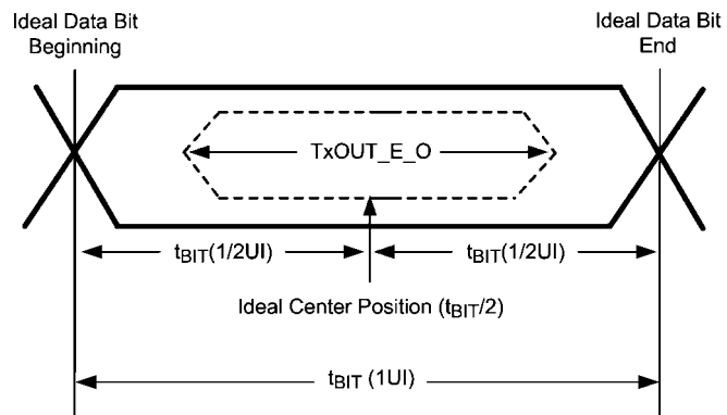
FIGURE 9. Transmitter Output Eye Opening ( \text{TxOUT\_E\_O} )
