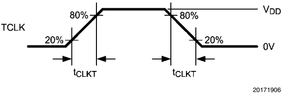
FIGURE 4. Serializer Input Clock Transition Times
