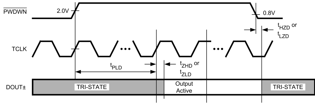
FIGURE 7. Serializer PLL Lock Time, and \text{TPWDNB} TRI-STATE Delays
