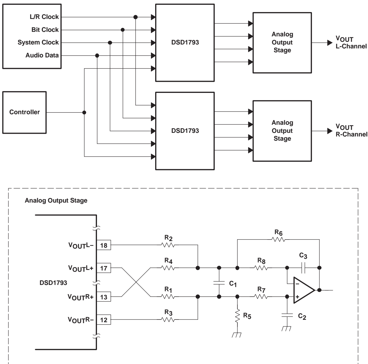
Figure 33. Connection Diagram for Monaural Mode Interface
