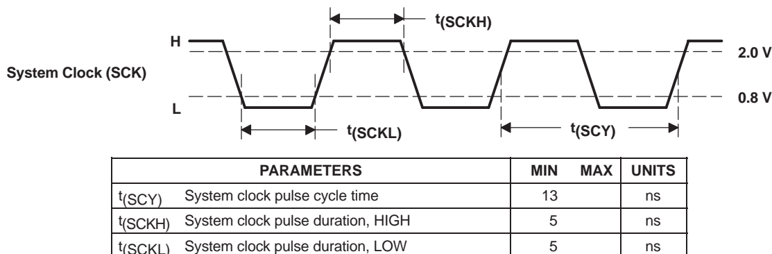
Figure 24. System Clock Input Timing
