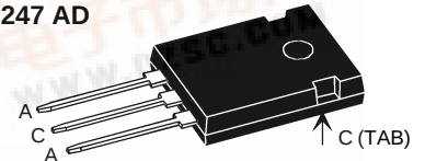
TO-247 AD
