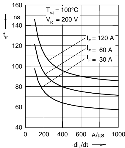
Fig. 5 Typ. recovery time t_{fr} versus -di_F/dt
