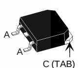
TO-268 AA (AT-Type)
