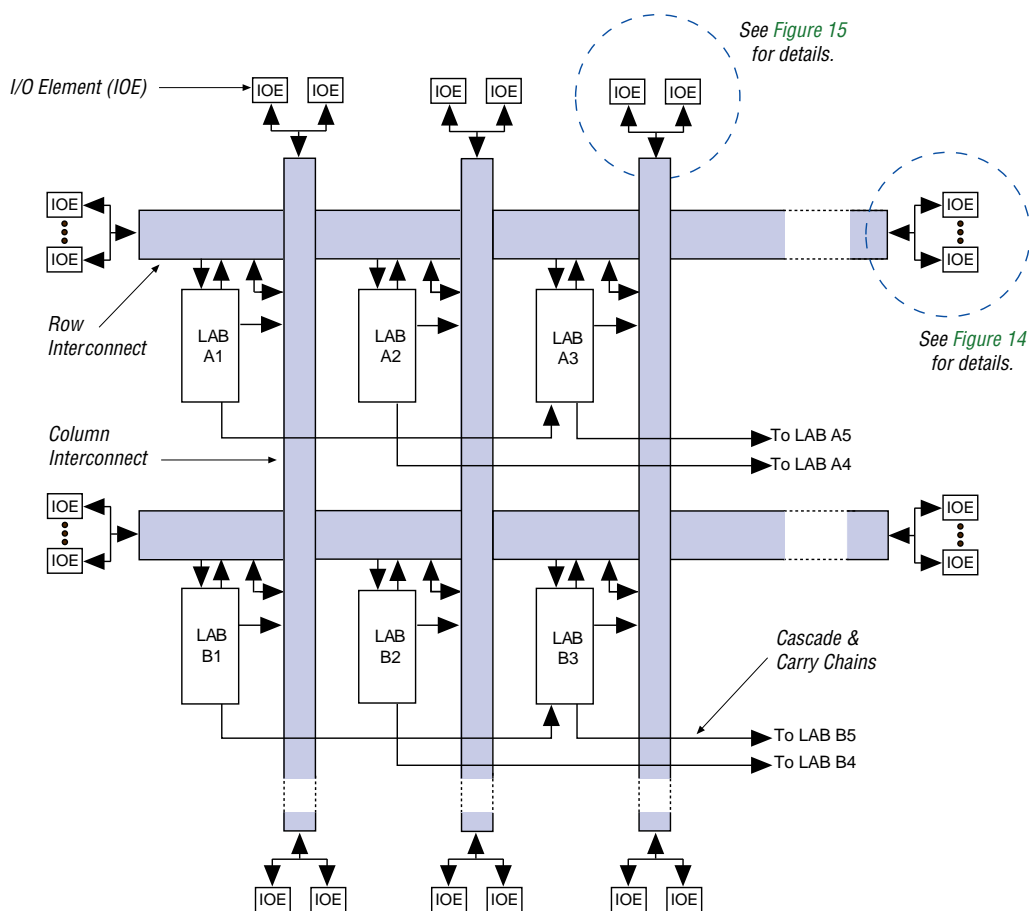
Figure 12. Interconnect Resources
