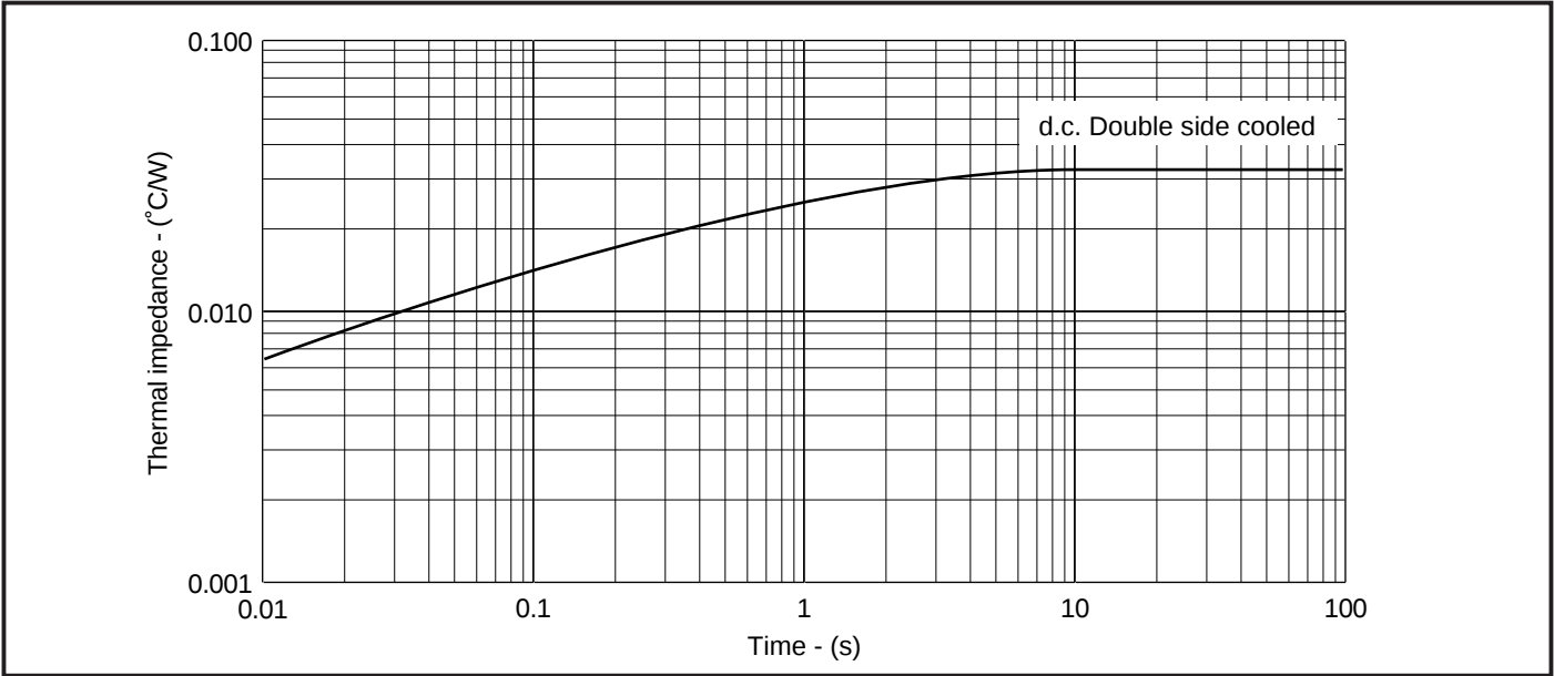
Fig. 3 Maximum (limit) transient thermal impedance - junction to case - ( ^{\circ}\text{C}/\text{W} )
