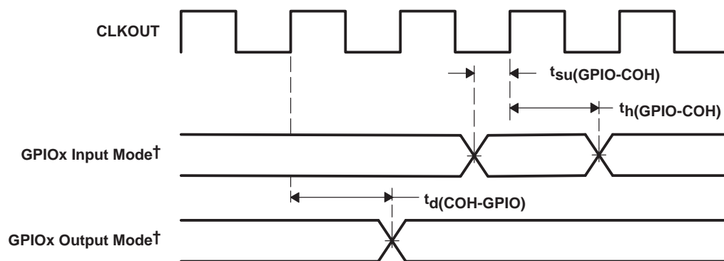
Figure 38. \text{GPIOx}^\dagger Timings
