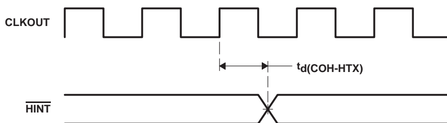
Figure 37. \overline{\text{HINT}} Timing
