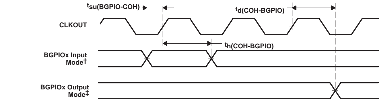
Figure 30. McBSP General-Purpose I/O Timings
