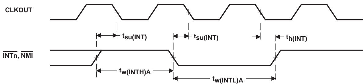
Figure 23. Interrupt Timing
