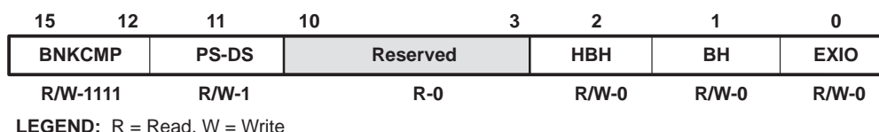
Figure 6. Bank-Switching Control Register (BSCR), MMR Address 0029h
