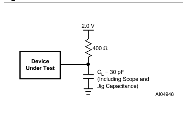
Figure 25. AC Measurement Load Circuit
