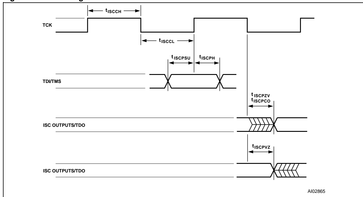
Figure 35. ISC Timing
