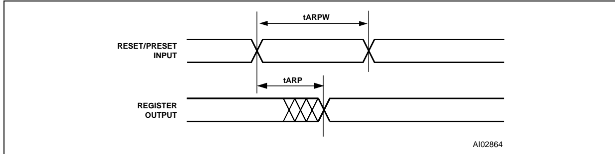
Figure 29. Asynchronous Reset / Preset
