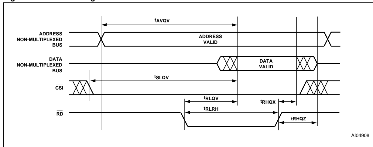
Figure 32. READ Timing
