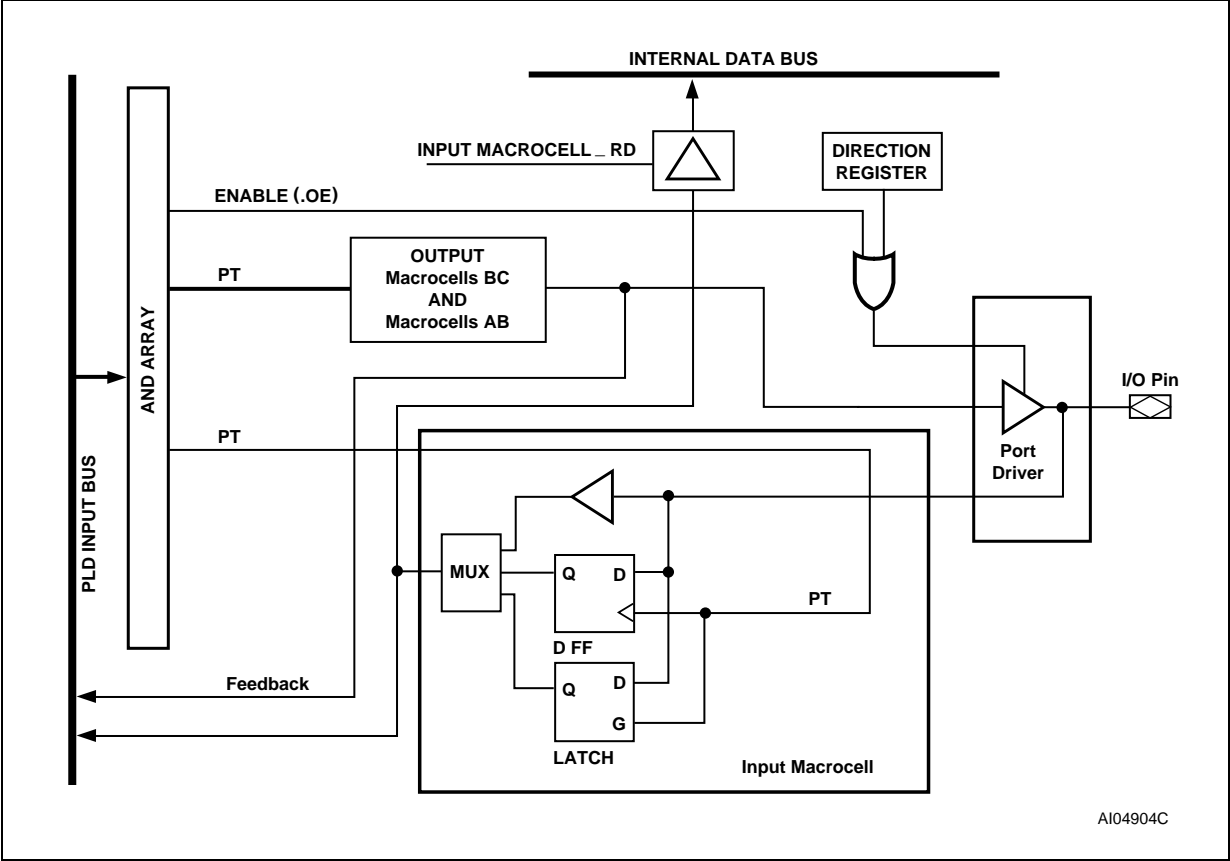
Figure 10. Input Macrocell
