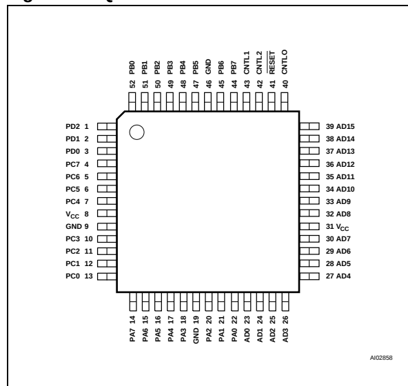
Figure 3. PQFP Connections
