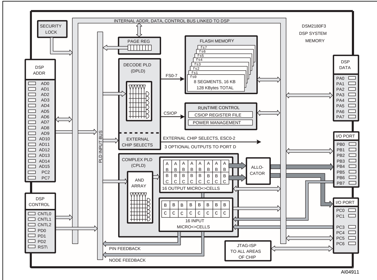
Figure 5. Block Diagram
