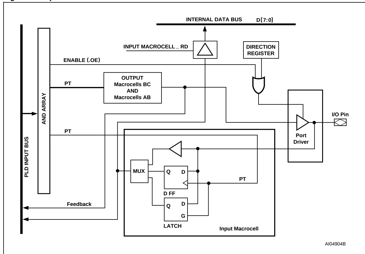
Figure 18. Input Macrocell
