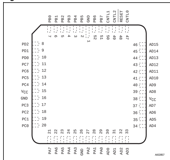
Figure 3. PLCC Connections
