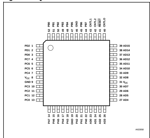
Figure 4. PQFP Connections
