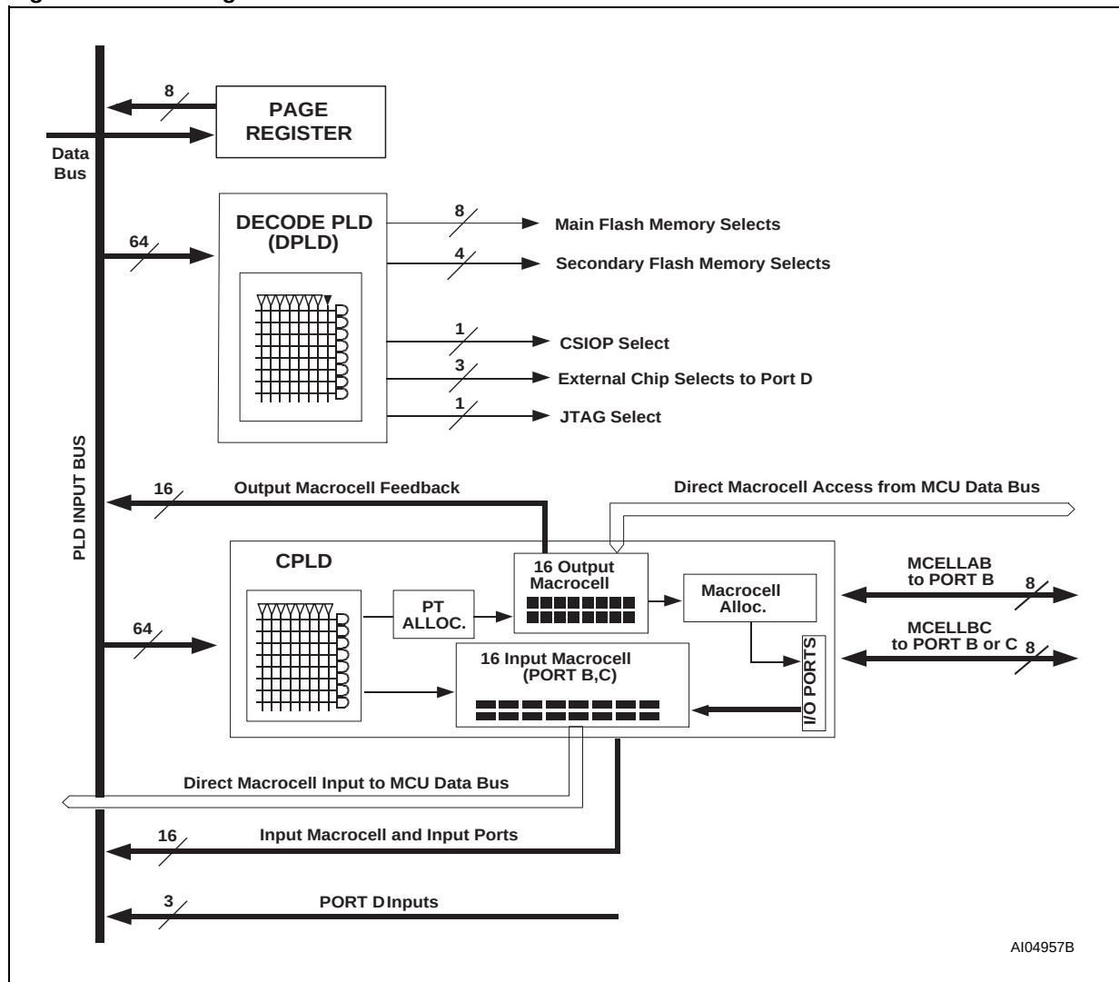
Figure 13. PLD Diagram
