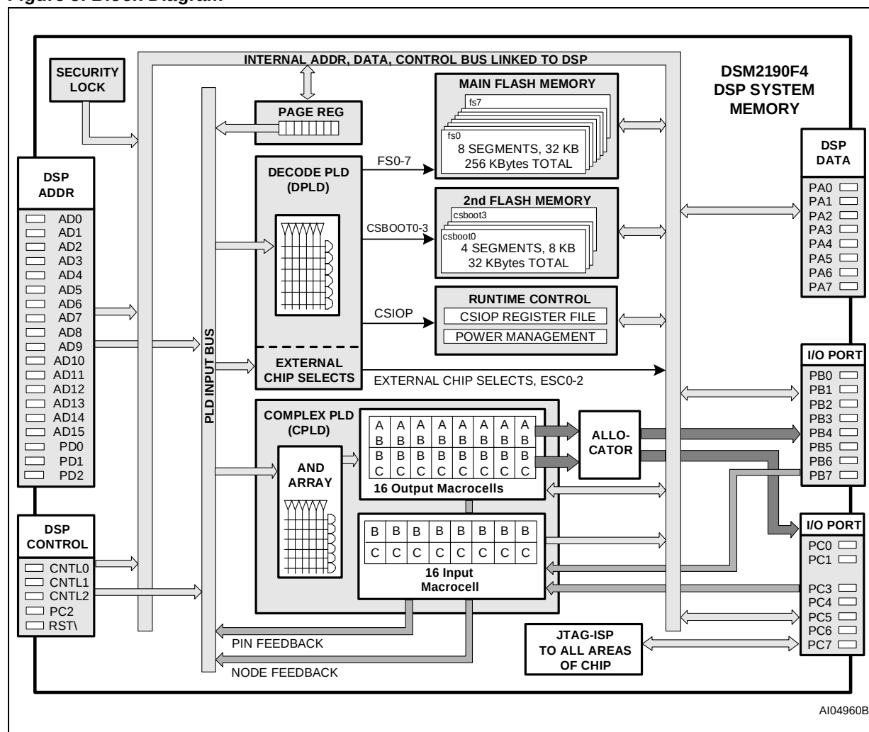
Figure 5. Block Diagram
