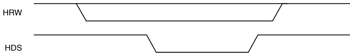
In a single-strobe bus, a DS (data strobe) signal qualifies the access, while a R/W (Read-Write) signal specifies the direction of the access.
