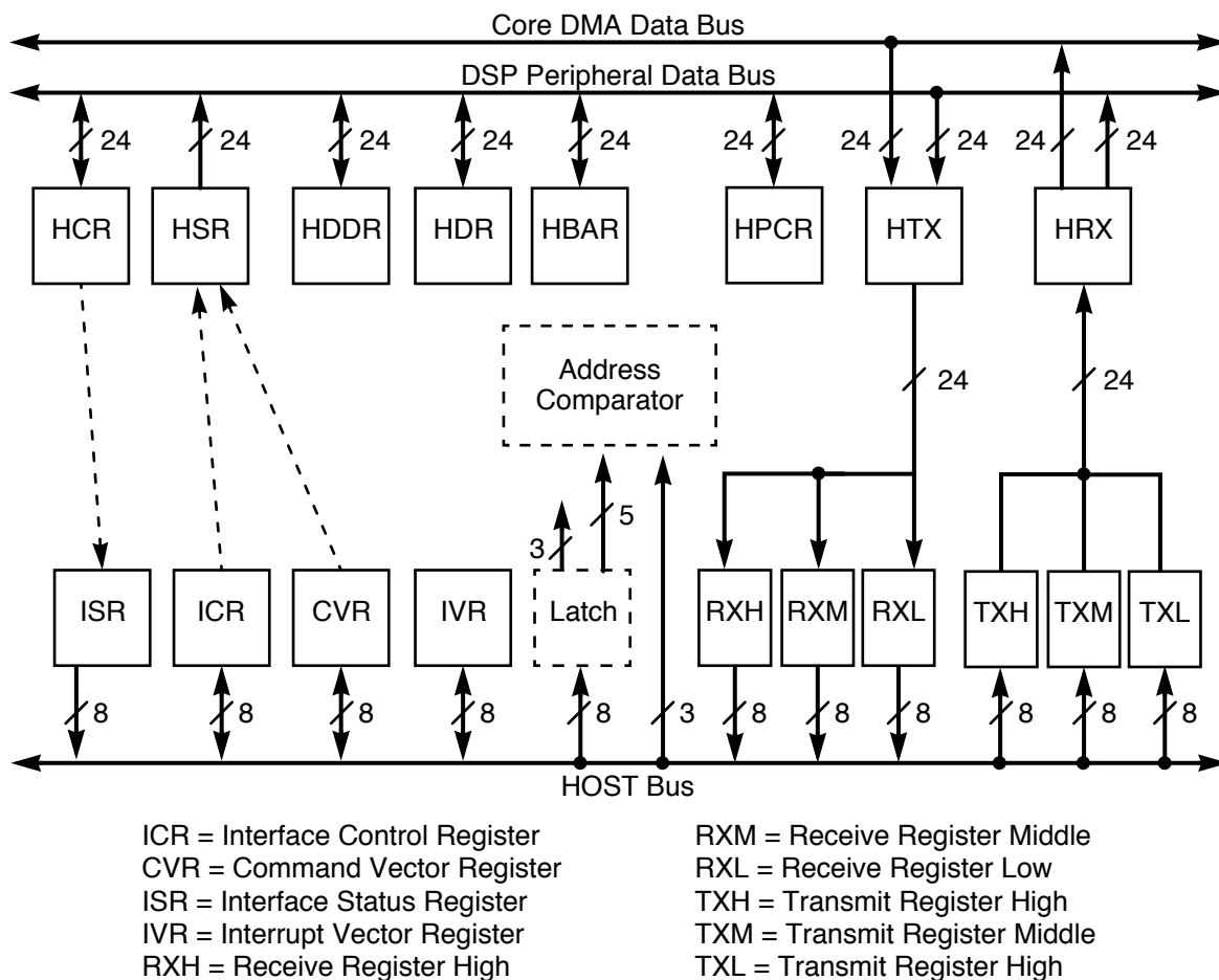
Figure 6-1 HI08 Block Diagram
