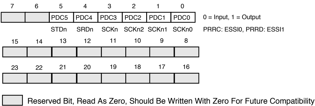
Figure 7-19 Port Direction Register (PRR)(PRRC X:$FFFFBE) (PRRD X:$FFFFAE)
