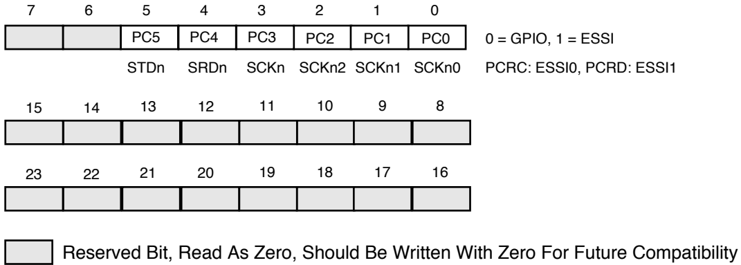
Figure 7-18 Port Control Register (PCR) (PCRC X:$FFFFBF) (PCRD X:$FFFFAF)
