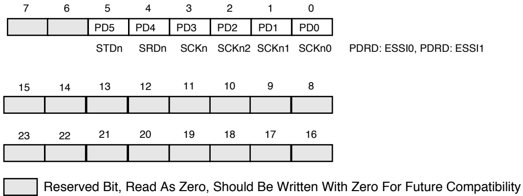
Figure 7-20 Port Data Register (PDR) (PDRD X:$FFFFBD)
