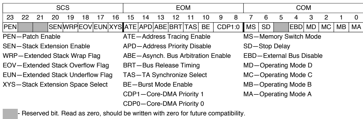
Figure 4-3 DSP56309 Operating Mode Register (OMR)
