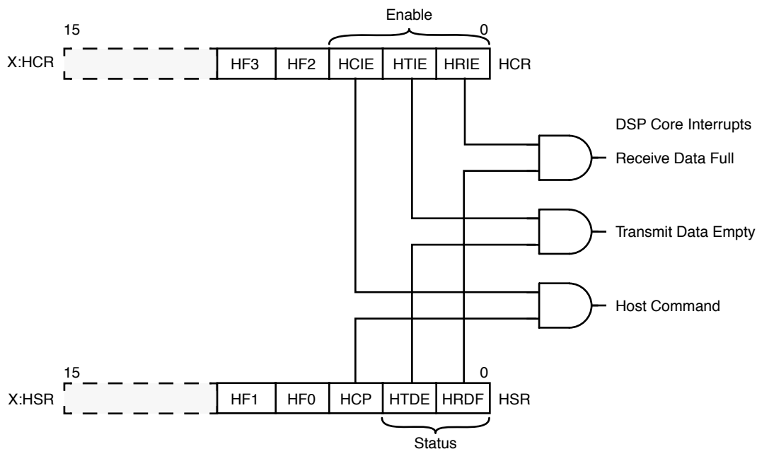
Figure 6-11 HSR-HCR Operation
