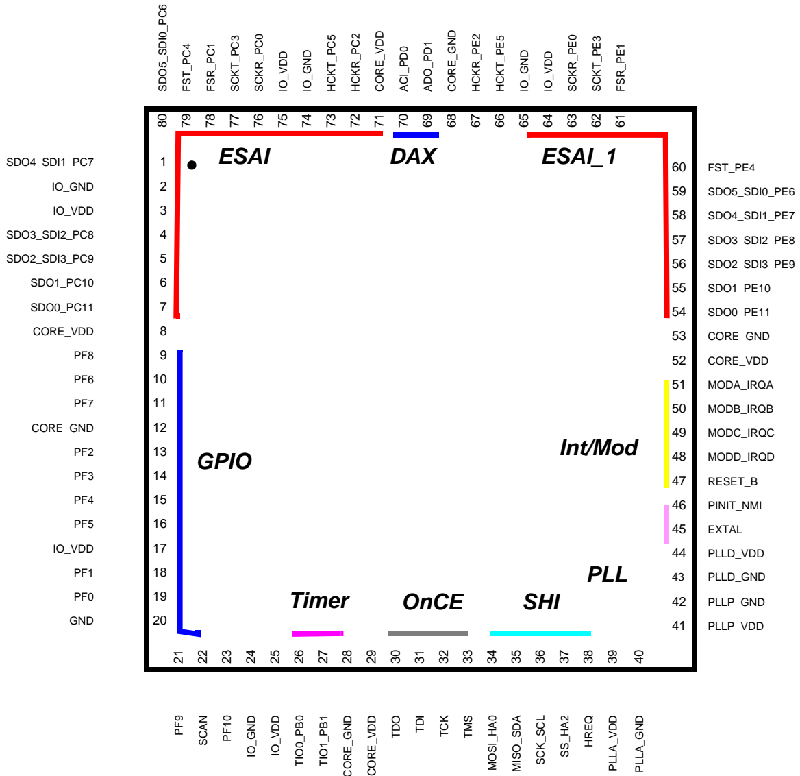
Figure 24. DSP56371 Pinout
