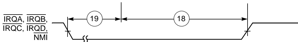
a) First Interrupt Instruction Execution
