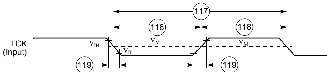
Figure 21. Test Clock Input Timing Diagram
