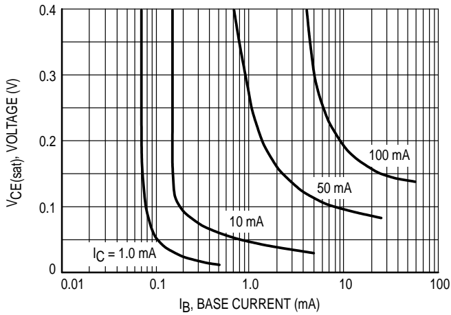
Figure 1. Collector-Emitter Saturation Voltage
