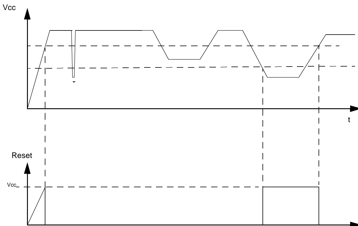
Figure 13. Power Fail Detect
