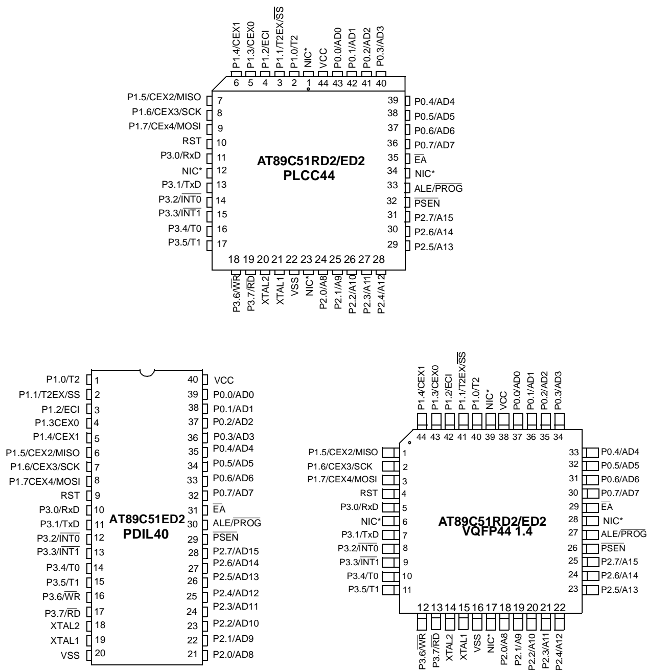
Figure 2. Pin Configurations
