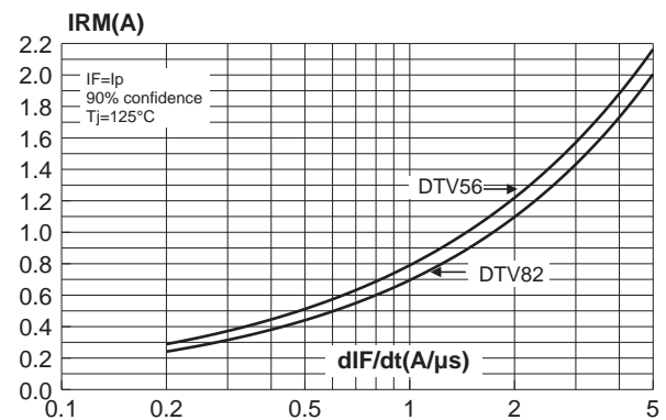
Fig. 6.3: Reverse recovery current versus dIF/dt.
