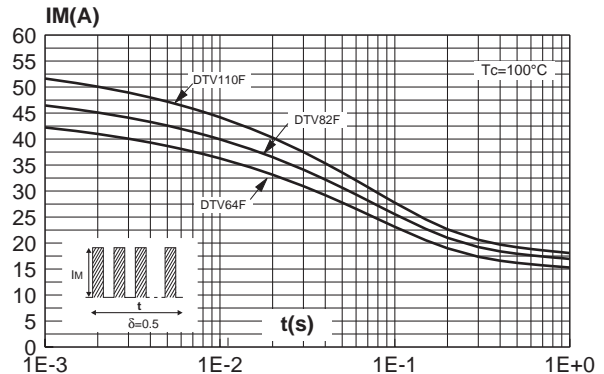
Fig. 4-4: Non repetitive surge peak forward current versus overload duration (ISOWATT220AC) (DTV64F / DTV82F / DTV110F).
