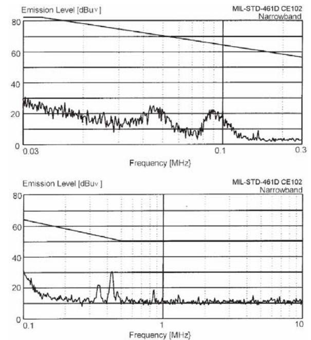
Figure 10 – MIL-STD-461D DVSA2800S With DVMA28 EMI Filter
