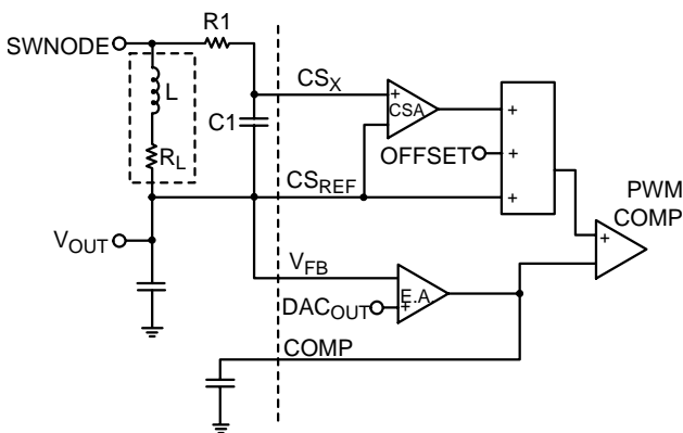
Figure 7. Lossless Inductive Current Sensing with Enhanced V^2
